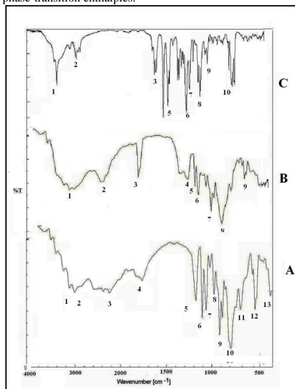
Figure 1 IR spectra of Carvedilol phosphate alone, physical mixture of polymers and drug-polymers combination
